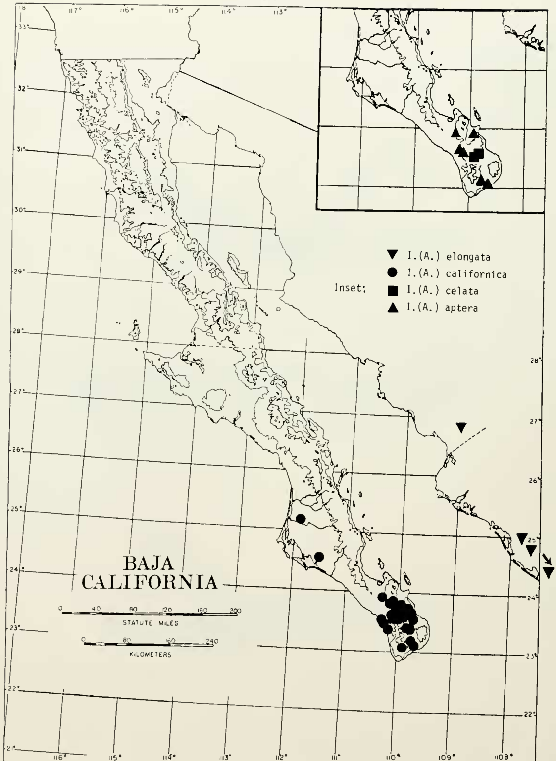
Figure 15. Known general distribution of Ichthiocris , subgenus Atyphacris , species other than I.(A.) costulata . Inverted triangles, I.(A.) elongata ; circles, I.(A.) californica ; squares (inset), I.(A.) celata ; upright triangles (inset), I.(A.) aptera .
